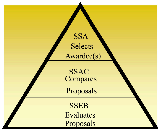
Figure 1-2: SST Responsibilities
